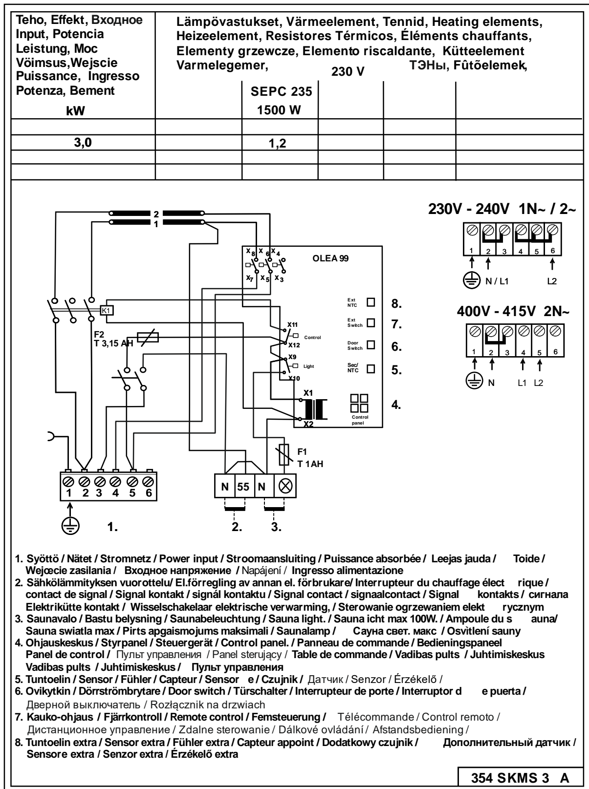
Figure 9 Wiring diagram for the sauna heater
