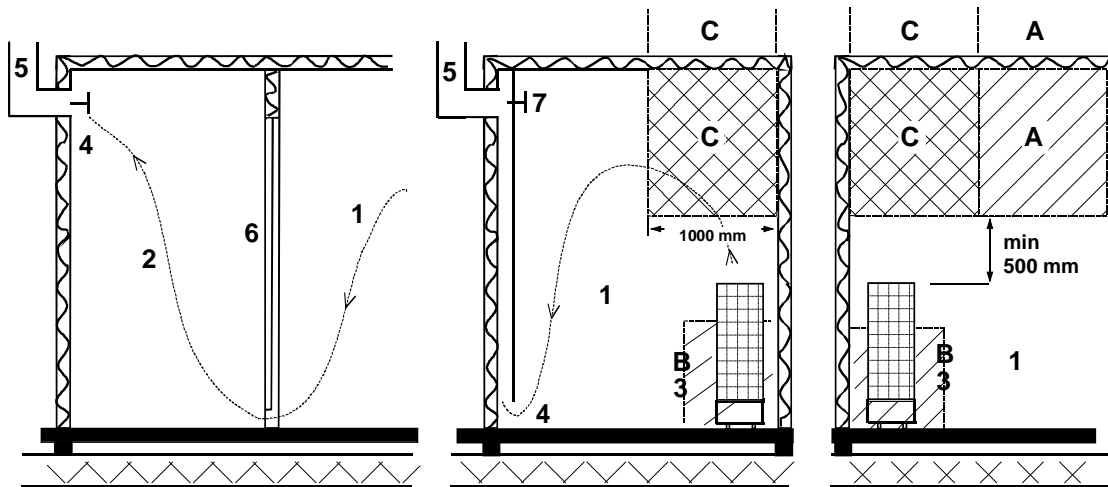
Figure 10 Recommended sauna room ventilation
