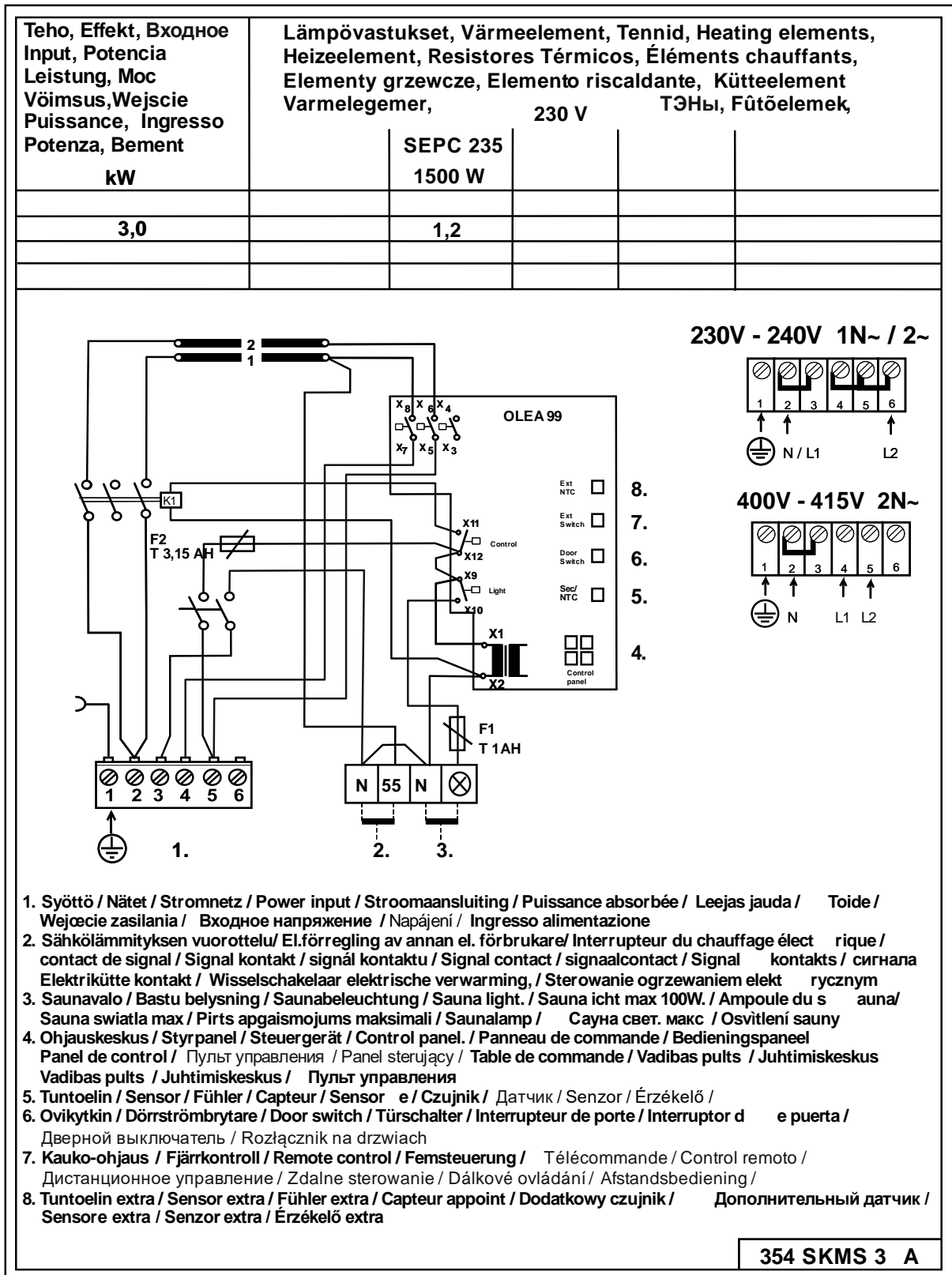
Figure 9 Schéma de raccordement
