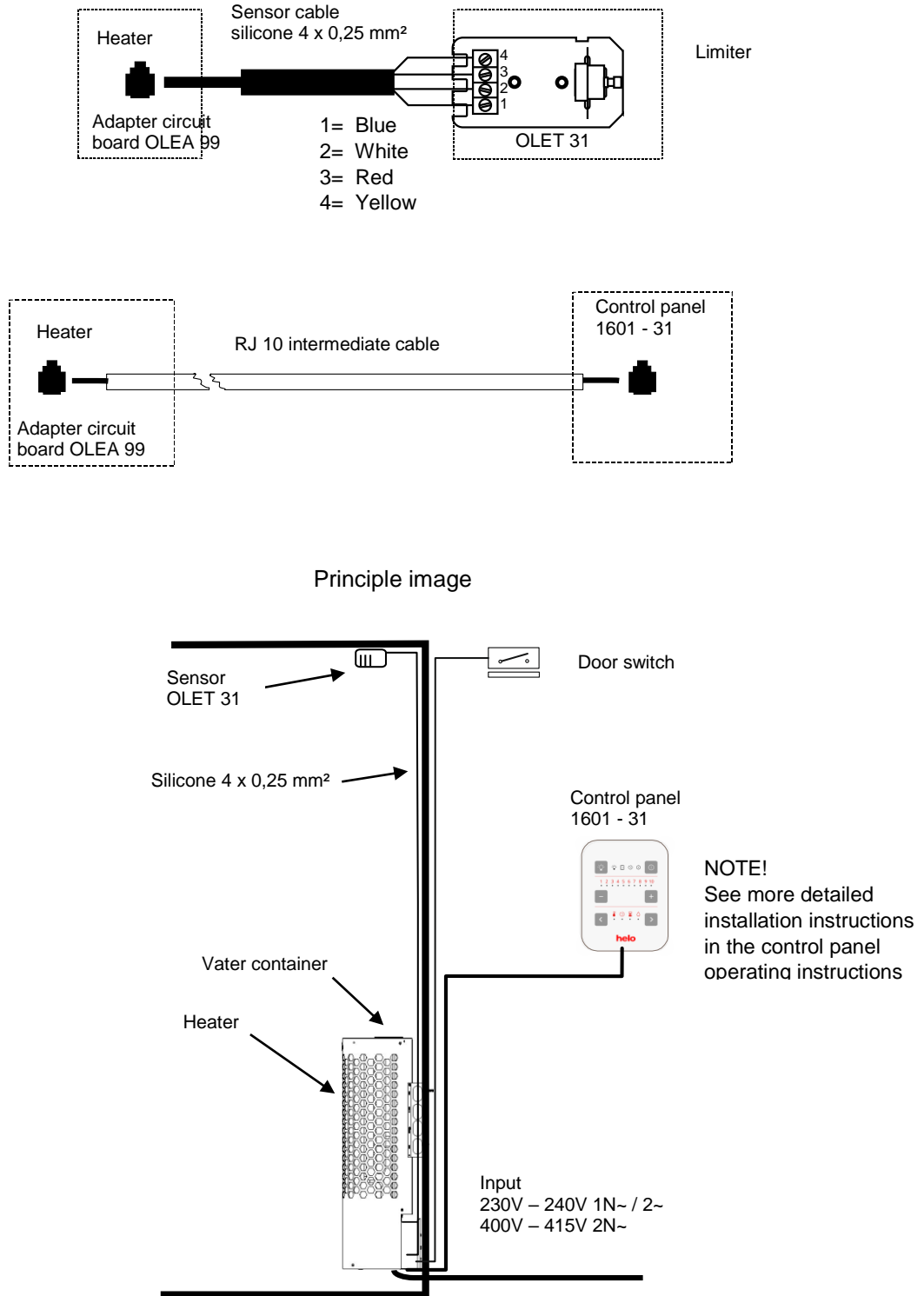
Figure 11 Principle image when 1601 - 31 (RA - 31 Trend) is used as control panel
