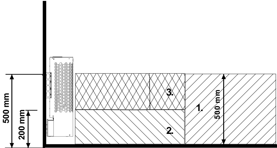
Figure 7 Location for the connection box
